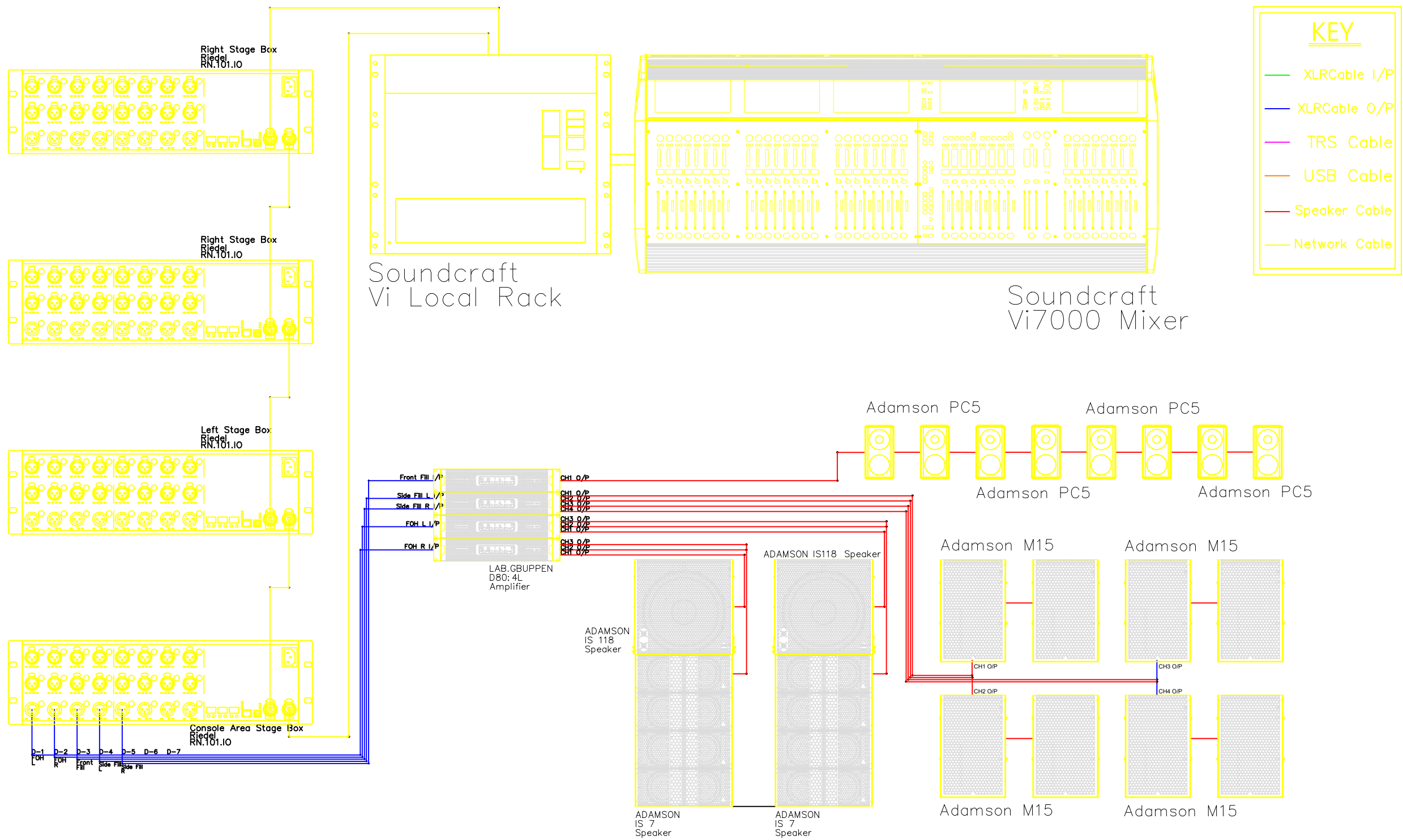
《 演藝中心音響系統圖 》 Draftsman : LIU,CHU-EN National Taiwan College of Performing Arts Performing Arts Center
